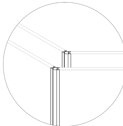
P4 Clear Polycarbonate Multi-angle Joint
