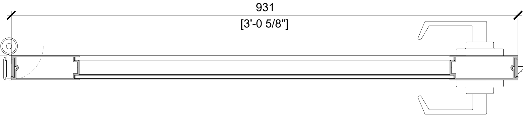
8 SWING D56 DOOR - HH45 - TERO SCALE: 1:4 (ON SIZE D - 34" X 22")
