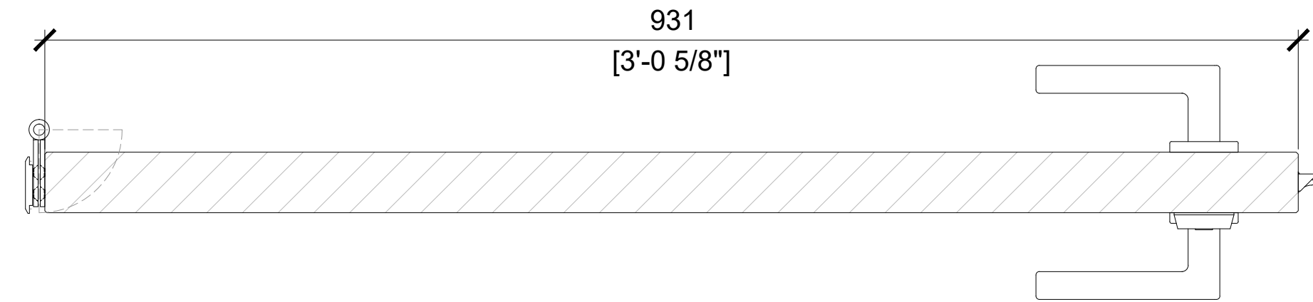
15 SWING WOOD DOOR - BH45 - REVEL SCALE: 1:4 (ON SIZE D - 34" X 22")
