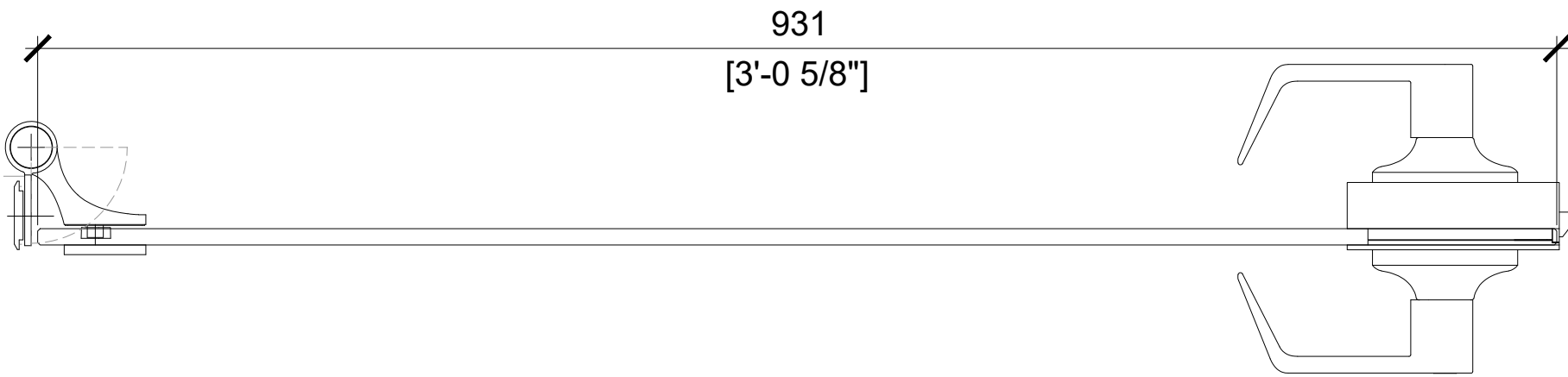
2 SWING FG10/12 DOOR - HHFG - SEJO SCALE: 1:4 (ON SIZE D - 34" X 22")
