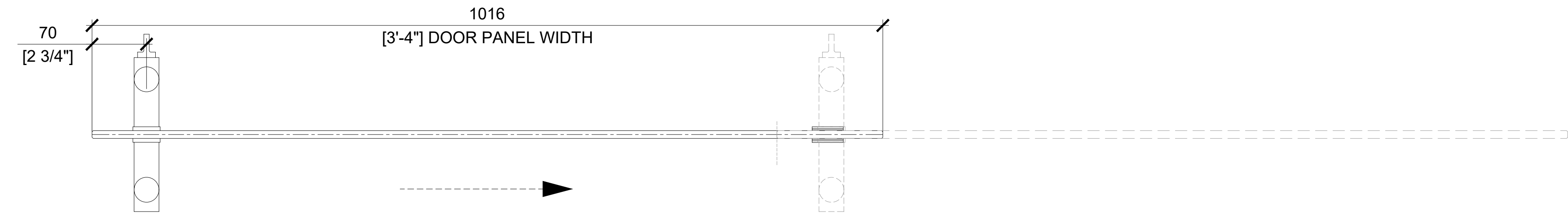
16 SLIDING FG10/12 DOOR - INTEC - KERE WITH 7 PIN SFIC LOCK SCALE: 1:4 (ON SIZE D - 34" X 22")
