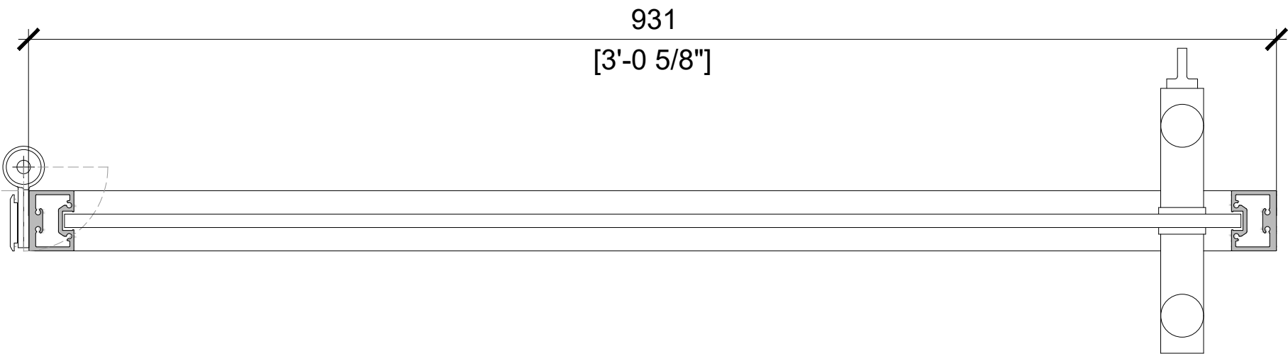
4 SWING S12 - HH45 - KERE SCALE: 1:4 (ON SIZE D - 34" X 22")
