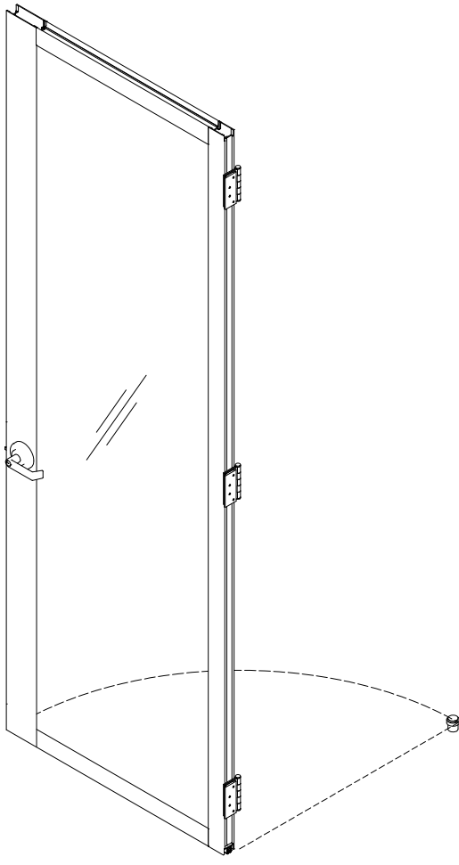
8 SWING D52 - TERO - BH45 SCALE: 1:20 (ON SIZE D - 34" X 22")
