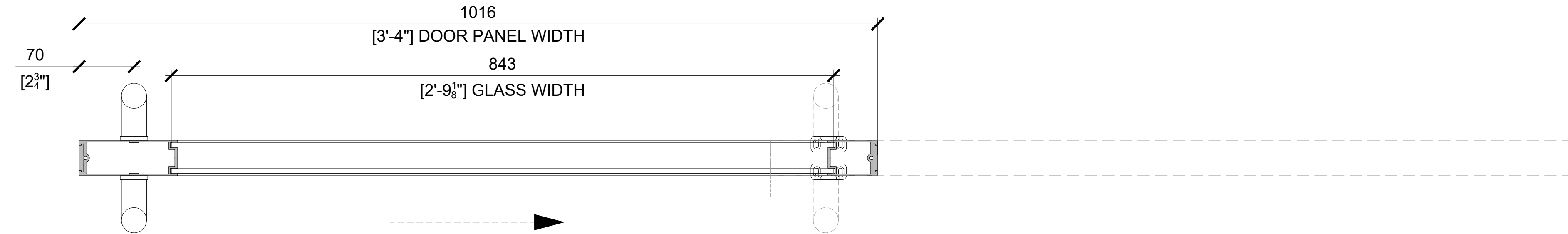
18 SLIDING D52 DOOR - INTEC - KERE NL SCALE: 1:4 (ON SIZE D - 34" X 22")
