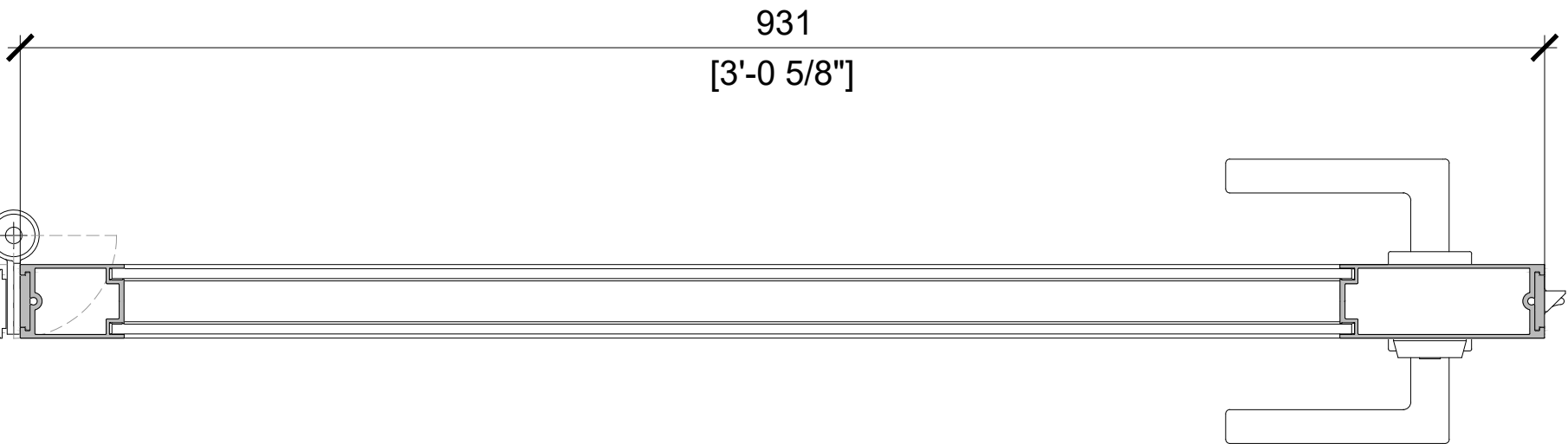
12 SWING D52 - HH45 - REVEL SCALE: 1:4 (ON SIZE D - 34" X 22")
