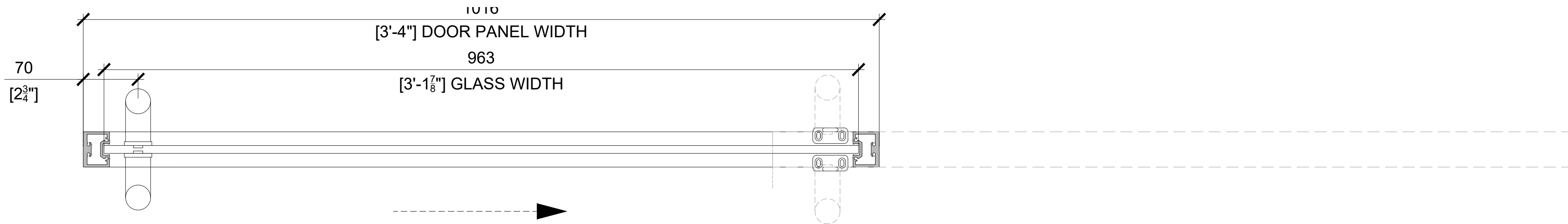
17 SLIDING S12 DOOR - INTEC - KERE NL SCALE: 1:4 (ON SIZE D - 34" X 22")
