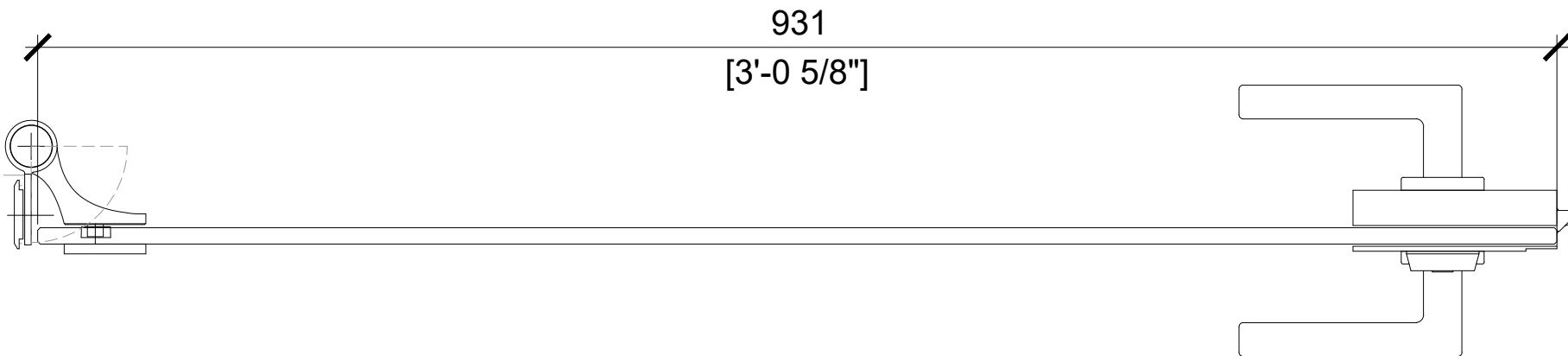
3 SWING FG10/12 - HHFG - SERE SCALE: 1:4 (ON SIZE D - 34" X 22")
