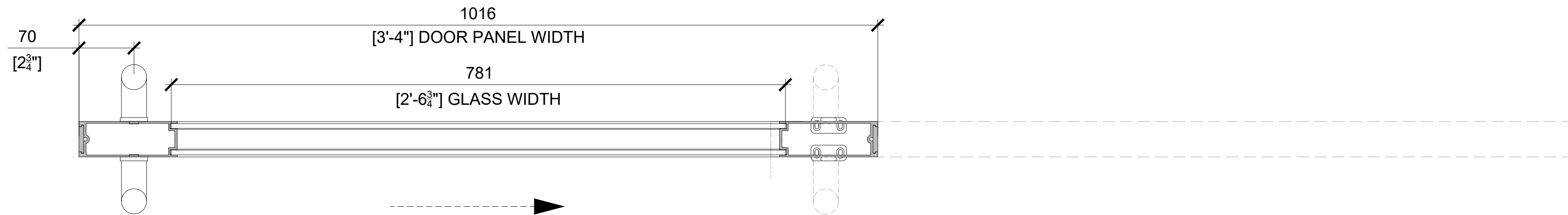
18 SLIDING D56 DOOR - INTEC - KERE NL SCALE: 1:4 (ON SIZE D - 34" X 22")
