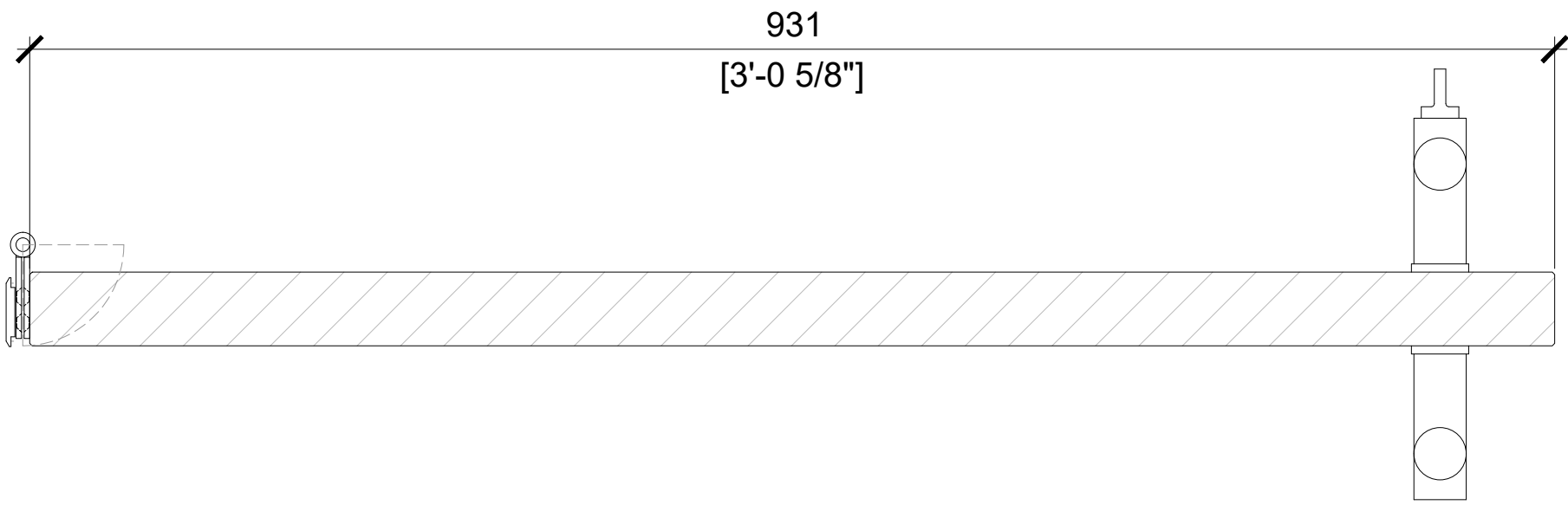
13 SWING WOOD DOOR - BH45 - KERE SCALE: 1:4 (ON SIZE D - 34" X 22")
