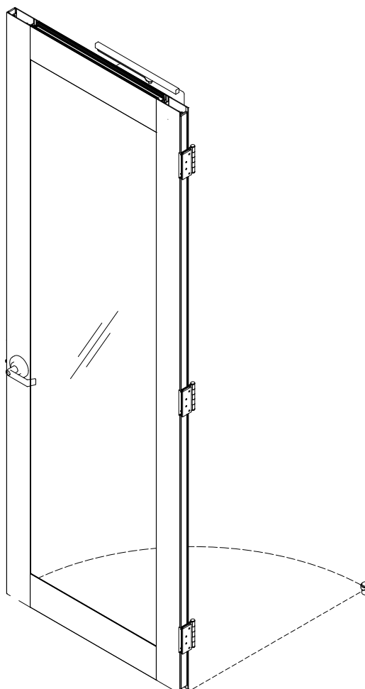
12 SWING D56 DOOR - TERO - BH45 SCALE: 1:20 (ON SIZE D - 34" X 22")
