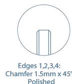
DETAIL BP SCALE 1 : 2
