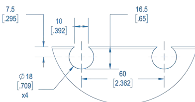
DETAIL BR SCALE 1 : 2
